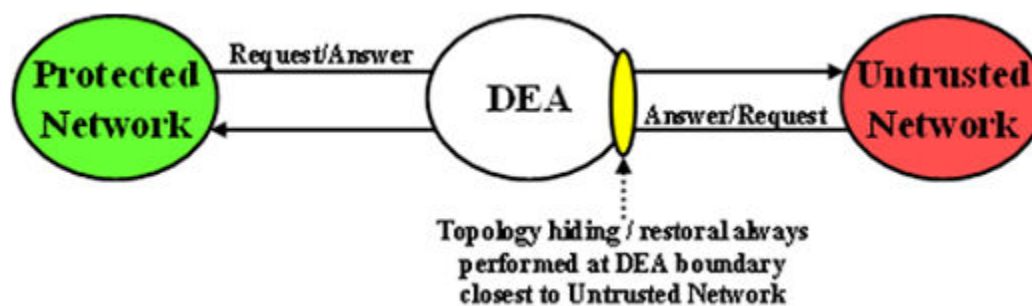
Figure 9-1 Diameter Topology Hiding Boundary
