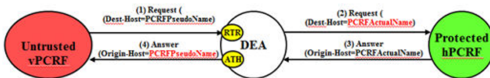
Figure 9-20 Untrusted-vPCRF to Protected-hPCRF Transaction
